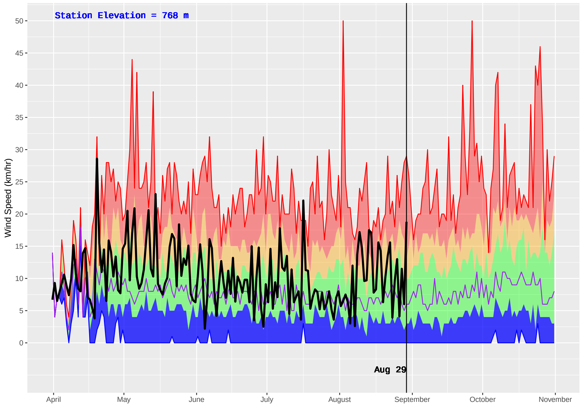
GRAHAM (124) : Historical (1979–2016) and Current (2018) Daily Wind Speed
