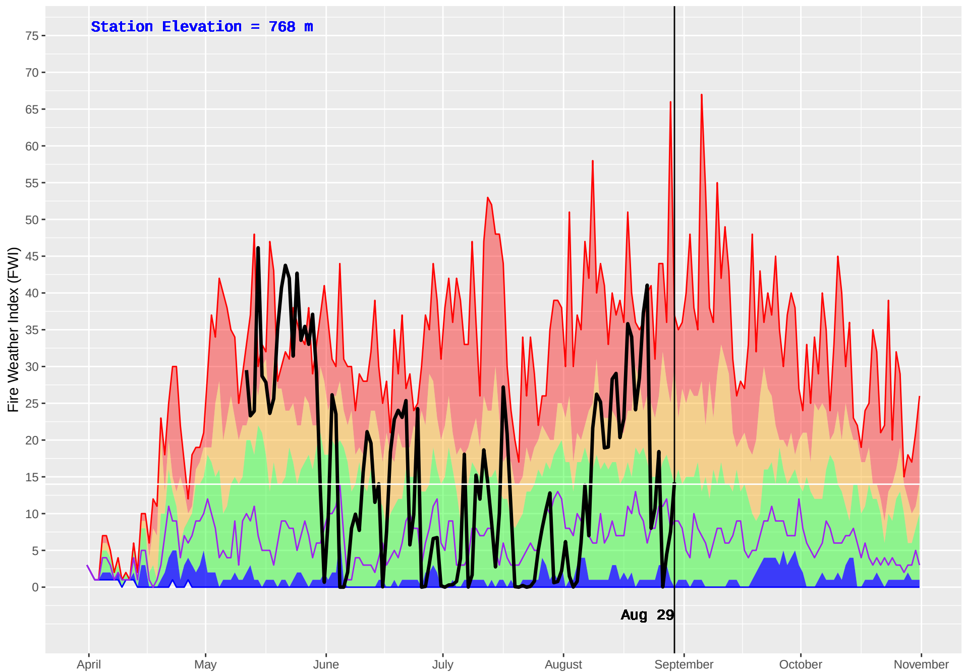
GRAHAM (124) : Historical (1979–2016) and Current (2018) Daily Fire Weather Index (FWI)
